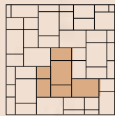
3-1-2 Herringbone Pattern 39% I's 9% II's 52% Magnum's
